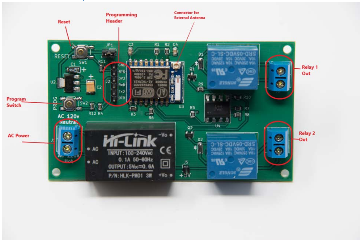
Figure 1-Hardware Breakout
